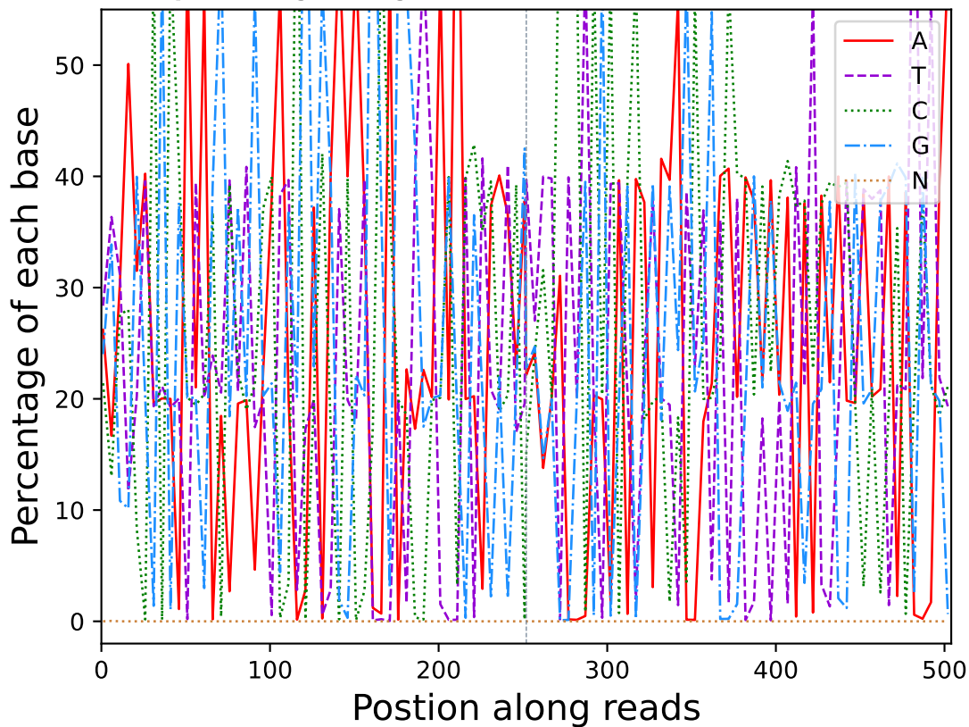
Base percentage along reads (R10508)
